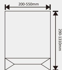
Gusseted Open -- mouth bag
