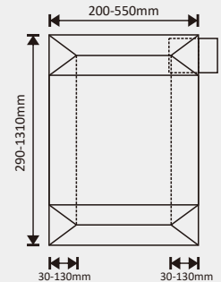
Gusseted Valve bag
