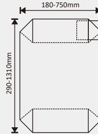
Valve bag
