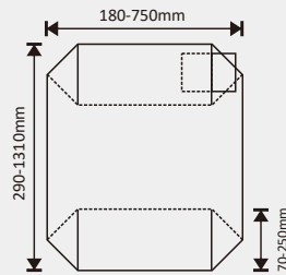
Valve bag - Regular size
